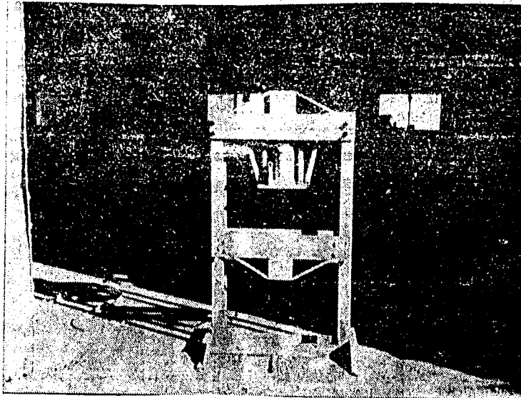
Completed 20 ton shop press by Jim Borcke
