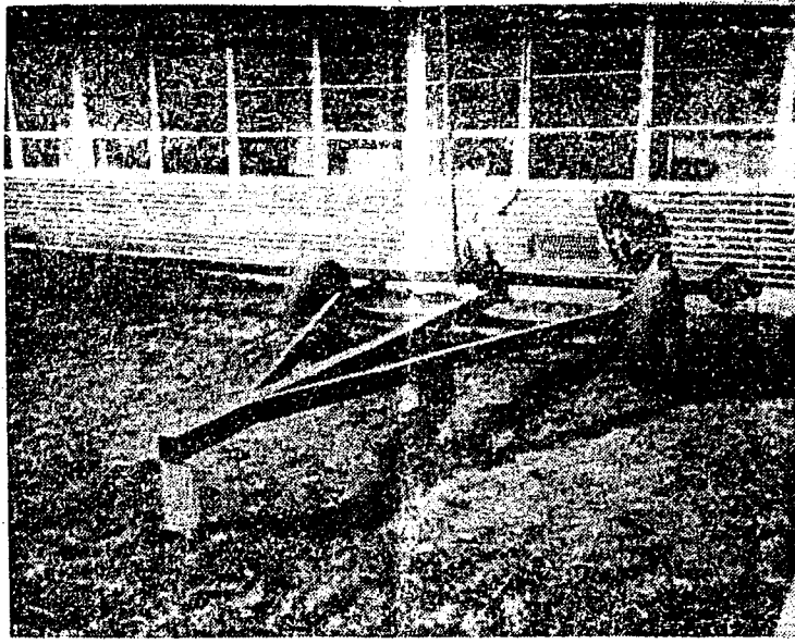
Harrow cart under construction by Gary Brammer
